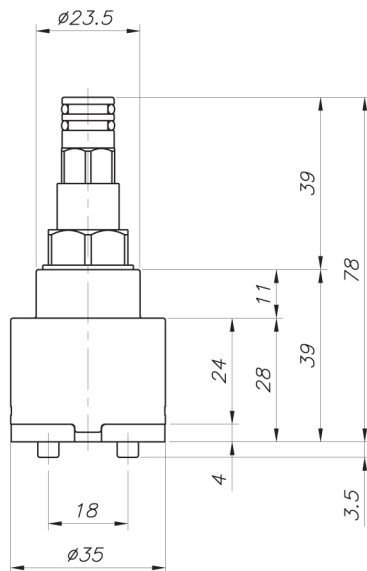
TPS35BD-2
