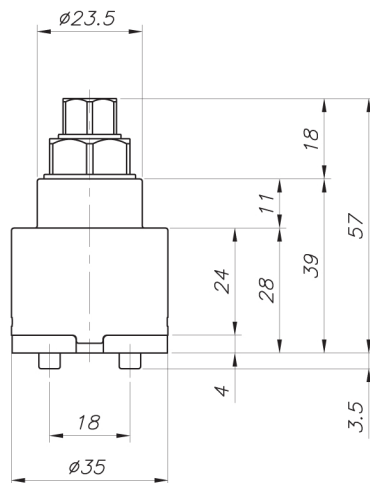
TPS35BD-1
