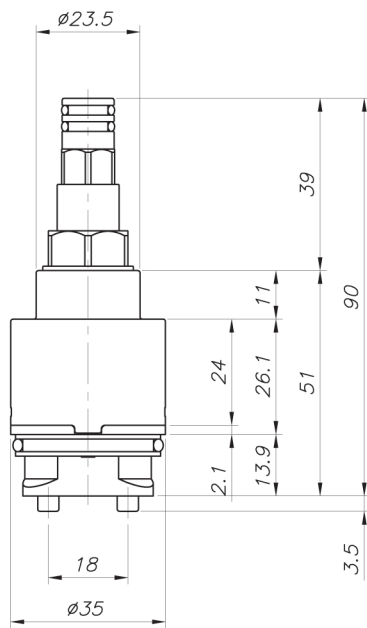
TPS35AD-2
