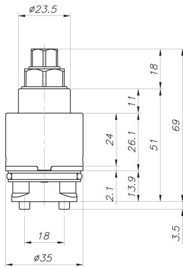
TPS35AD-1
